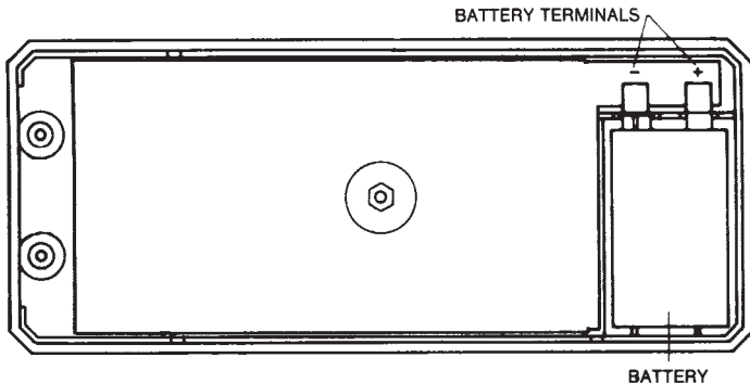
Figure 2 Battery Installation
